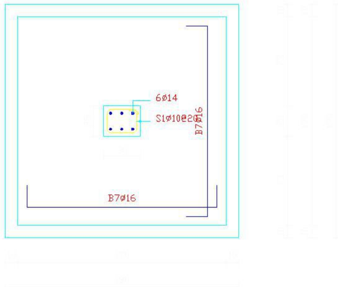
SEC. IN F1C1 1:20
