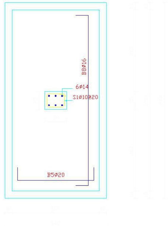
SEC. IN F2C1 1:20
